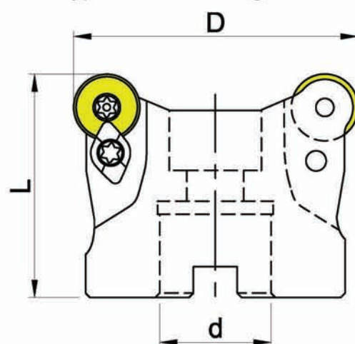
RM R- Type Surface Milling Cutter
