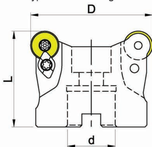
RW R- Type Surface Milling Cutter
